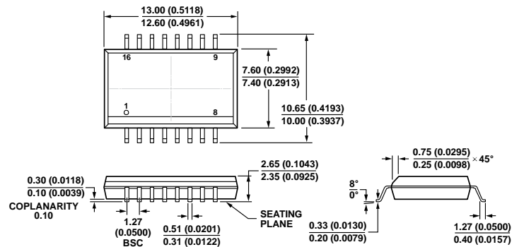
Figure 19. 16-Lead Standard Small Outline Package [SOIC_W] Wide Body (RW-16)
